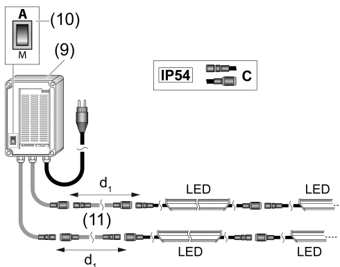
Figure 7: Degree of protection IP64 / Connection type C
