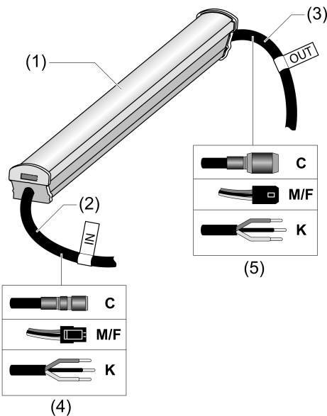
Figure 1: LED luminaire LEDLUX LN linear
