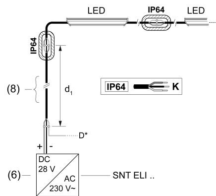
Figure 6: Degree of protection IP64 / Connection type K
