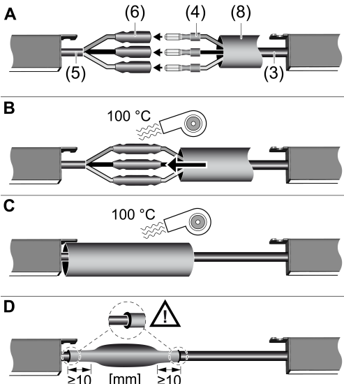
Figure 6: Linking LED lamps
