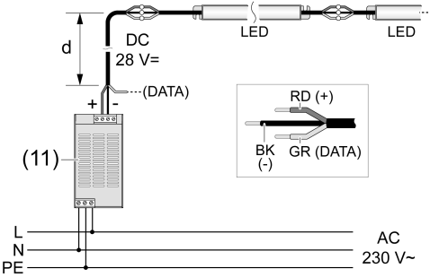
Figure 5: Circuit diagram
