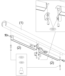
Lichteins a tze montieren Installing lighting inserts
