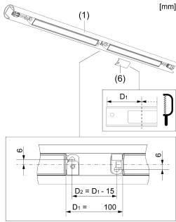
Abstand festlegen + Nutabdeckung anpassen Determining distance + adapt groove cover
